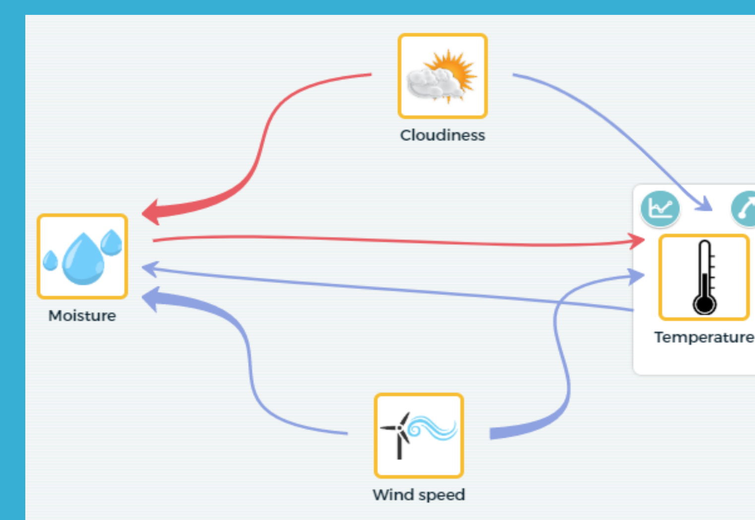
Scientific Modeling
