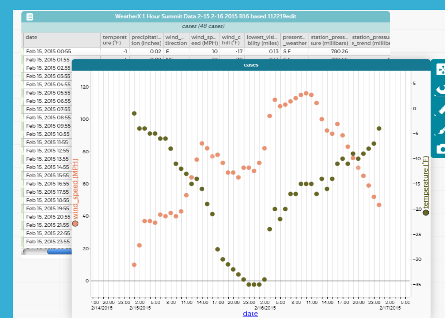
Big Data
